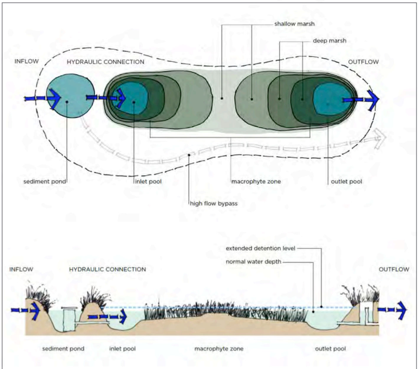
FIGURE 2 Schematic Layout of a Constructed Wetland System
