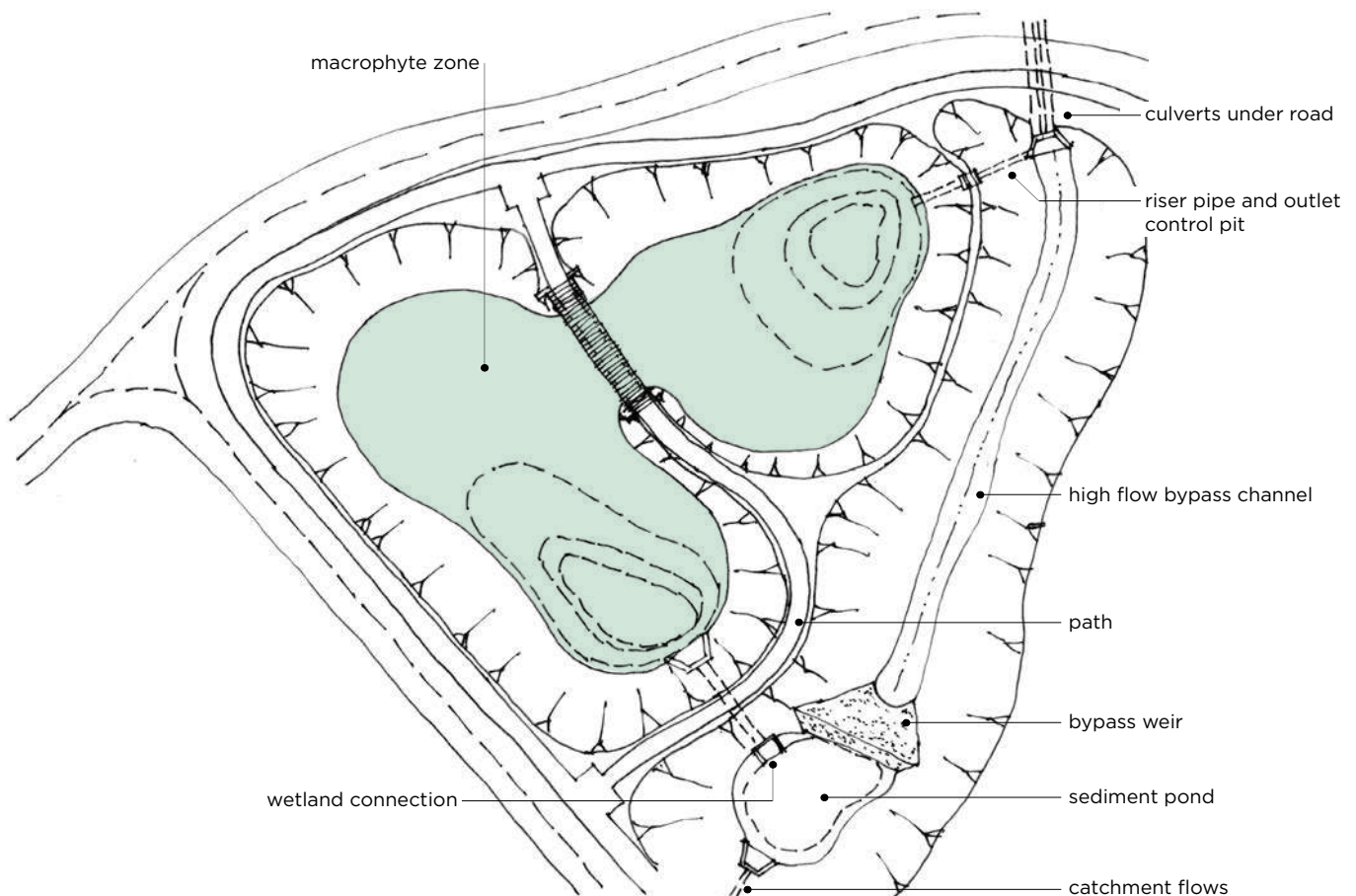
FIGURE 46: Layout of Proposed Wetland System
