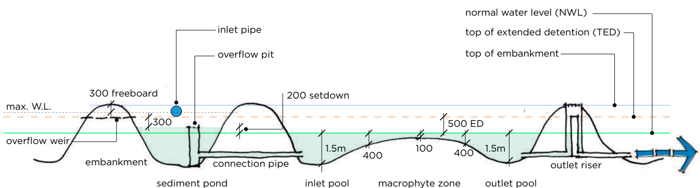
FIGURE 6 Extended detention depth and maximum water level requirements
