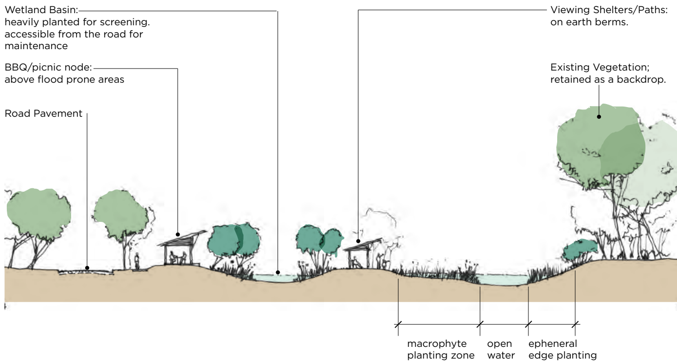
FIGURE 9 Typical landscape treatments to constructed wetlands in open space areas
