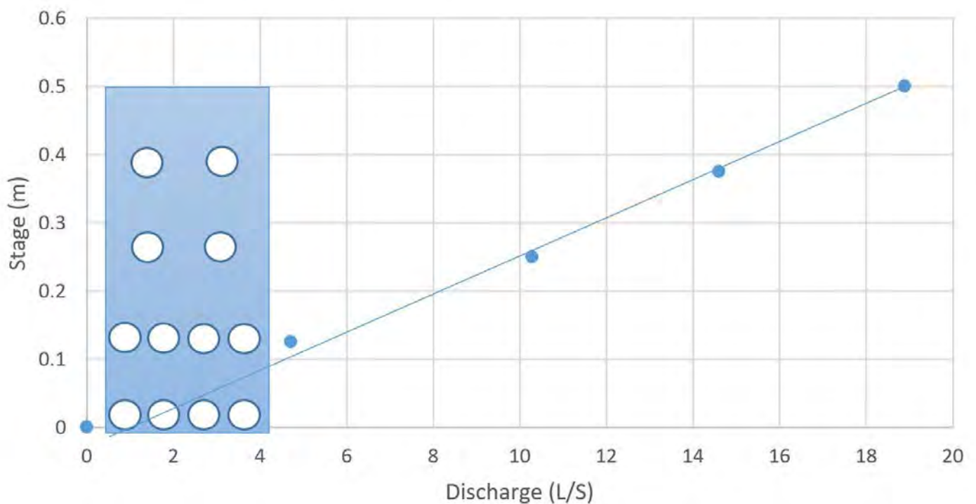
FIGURE 48 Riser Pipe Configuration Showing Discharge Stage Relationship
