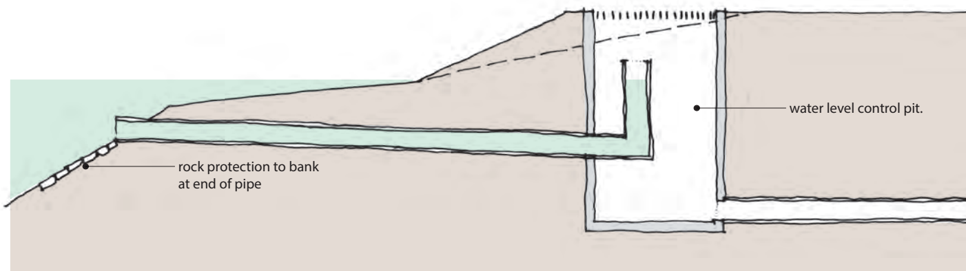
FIGURE 30: Typical Macrophyte Zone Outlet Arrangement
