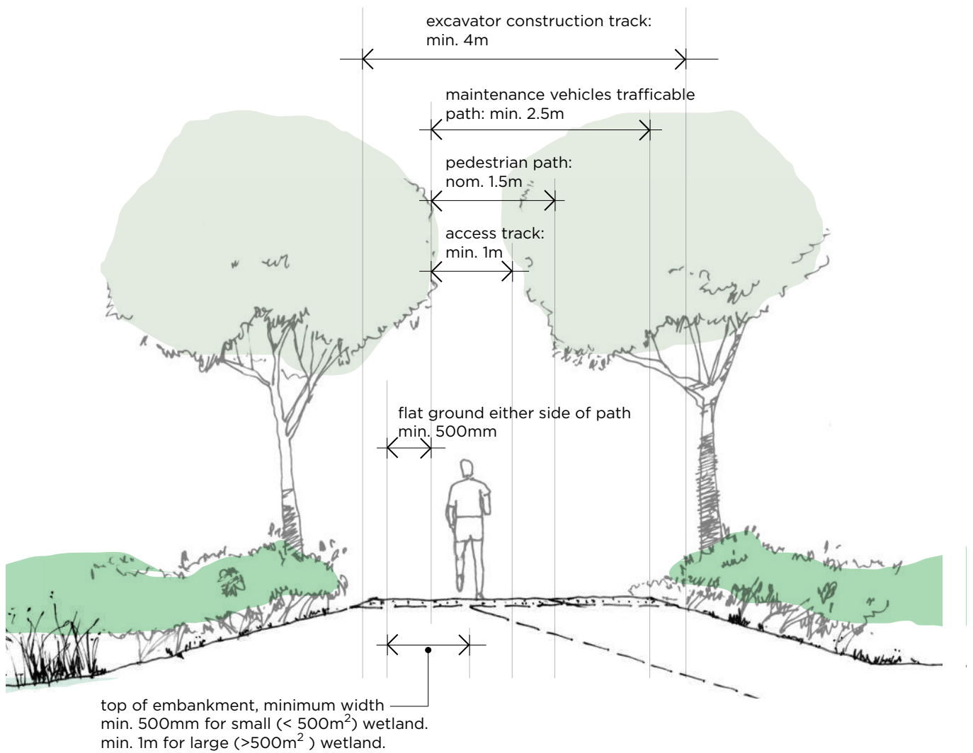
FIGURE 29 Embankment width requirements
