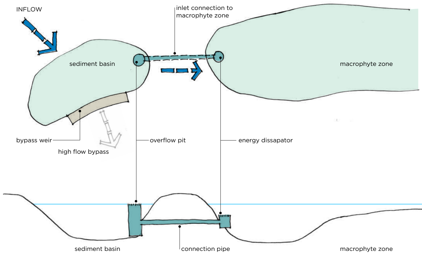
FIGURE 16 Example of sediment basin connection to macrophyte zone
