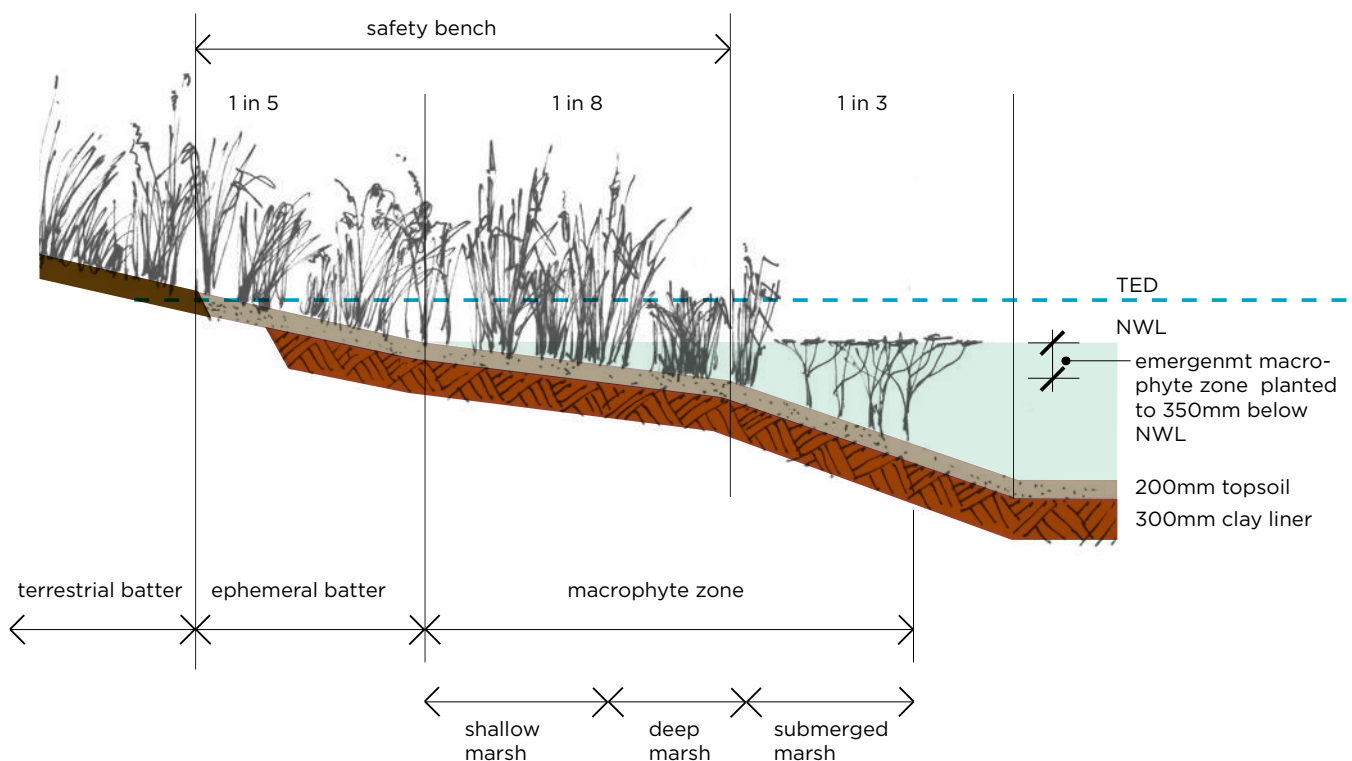
FIGURE 42 Wetland planting zones
